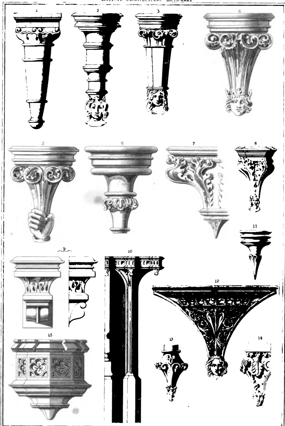
BRACKETS. 1. Buildwas Abbe Church. 2. St. Mary, Overgate, Ch. Southwark. 3. Wells Cath. Crypt under Chap. House. 4. Laycock, Abbe Wilts. 5. Lady Chap. York Cath. 6. Winton, Ch. Wilts. 7. Leas, Ch. Cant. Cath. 8. Chepstow Castle. 9. Entrance to Chap. House. 10. Wells Vault. 11. St. Alb. Hall, London. 12. 13. 14. 15. (Additional drawings) London, Published by Messrs. Dean & Deane, 1858.
