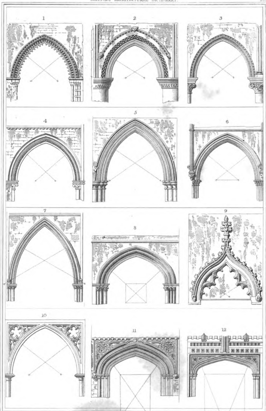
1. Walsoken Ch. Nave. 2. Malmesbury Abb. Choir. 3. Canter? Cath. Choir. 4. Canter? Cath. S.E. Transept. 5. Salisbury Cath. Nave. 6. Lincoln Cath. Nave. 7. York Cath. 8. Chester Cath. 9. Westm? Abb. Cloisters. 10. Canter? Cath. Nave. 11. Canby, K.C. Chap. 12. Crosby Hall.
